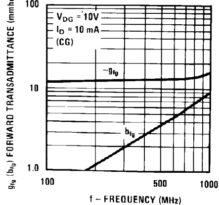
Forward Transadmittance
